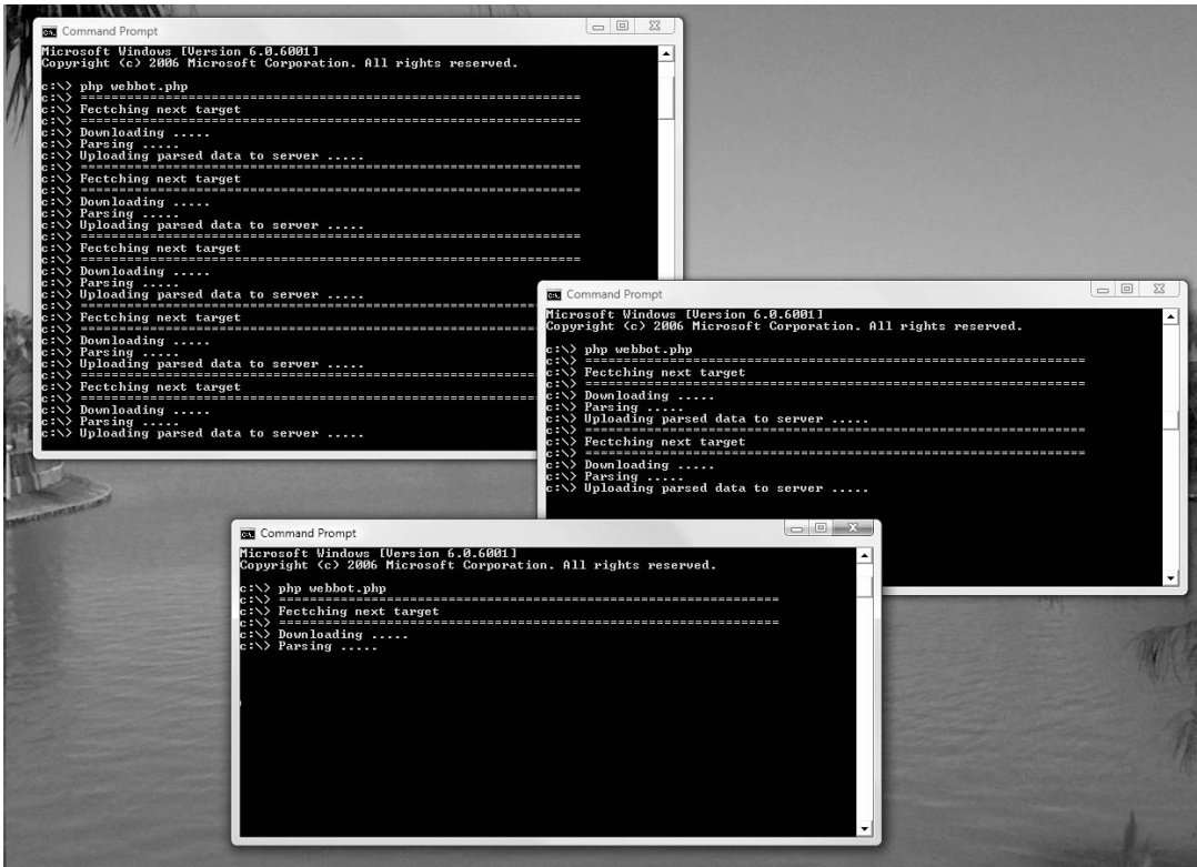
Figure 25-5: Using the operating system to create multiple instances of a webbot
