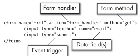
Figure 6-2: Parts of a form
