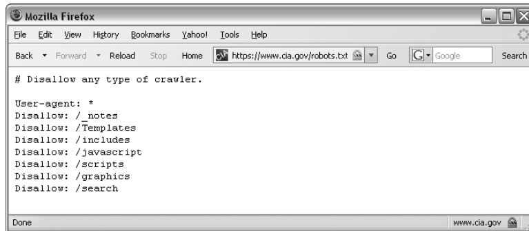
Figure 30-1: A typical robots.txt file, disallowing all user agents from selected directories
