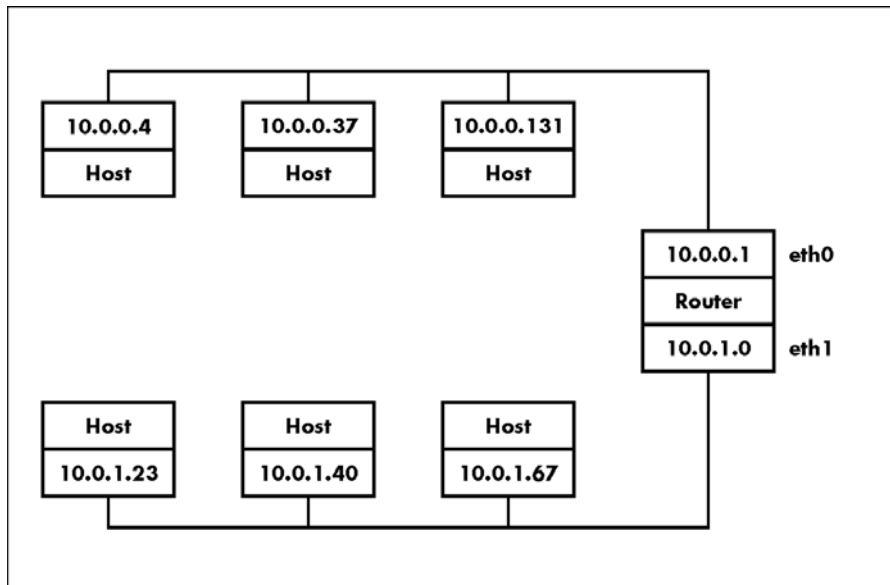
Figure 5-4: Two subnets joined with a router.
