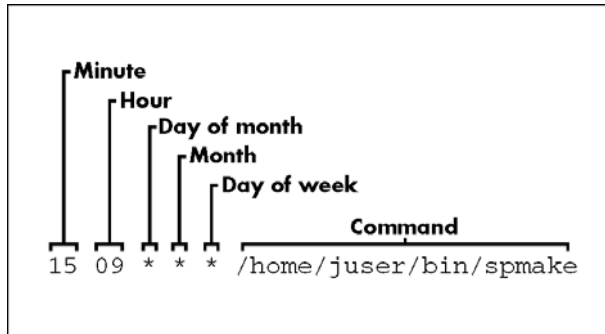
Figure 4-3: An entry in the crontab file.
