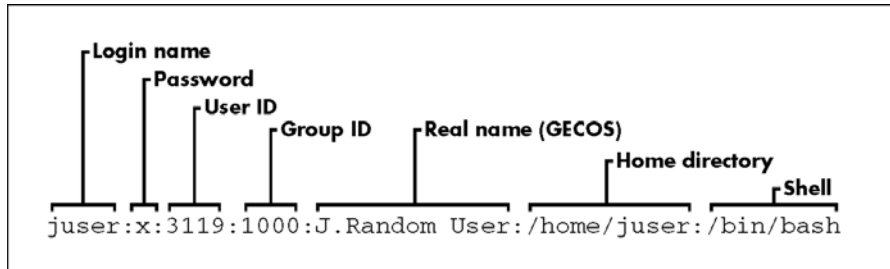
Figure 4-1: An entry in the password file.
