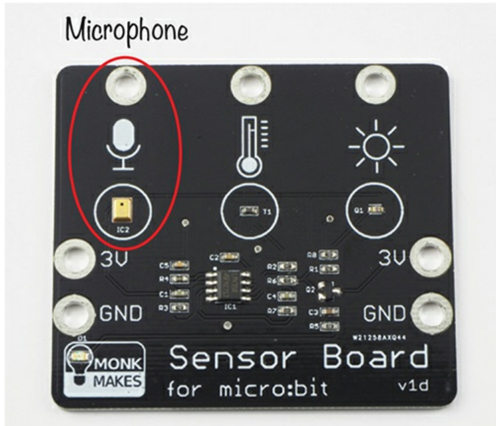
Figure 2-9: The Monk Makes Sensor for micro:bit microphone
