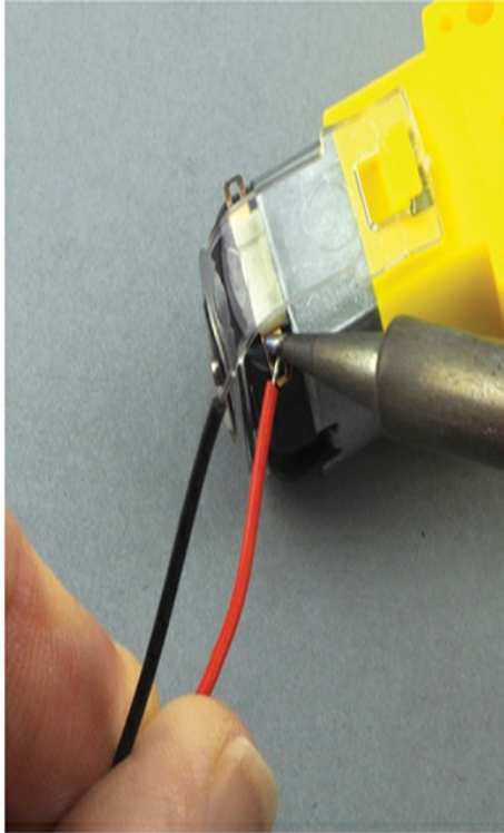
a. Soldering the first motor wire
