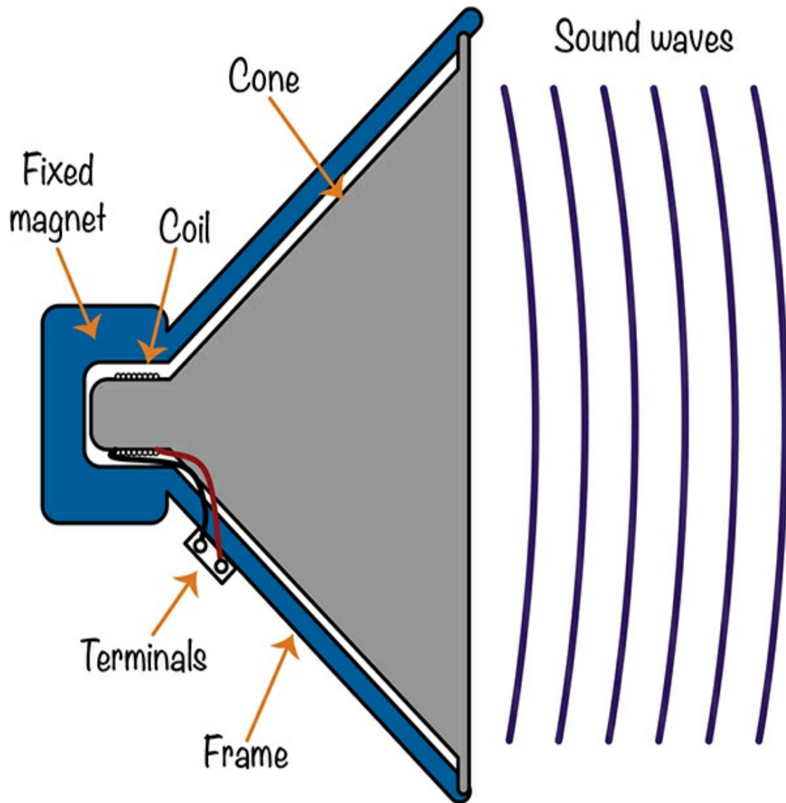
Figure 2-5: A loudspeaker
