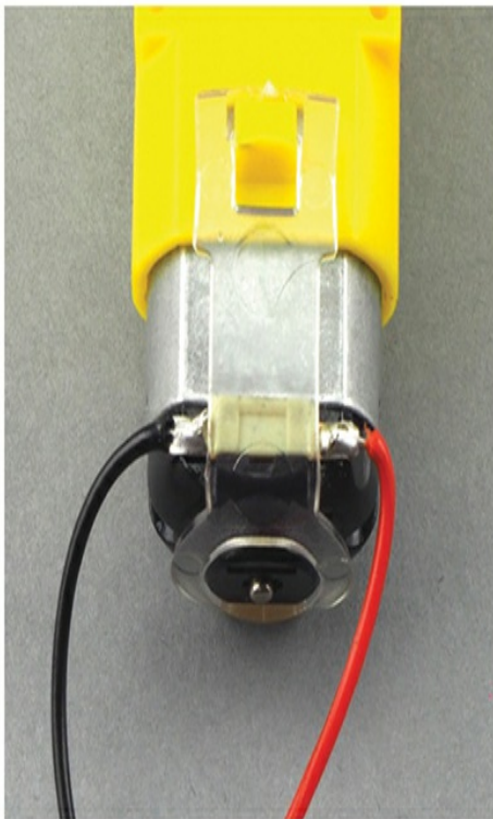
c. Both wires soldered to the gearmotor
