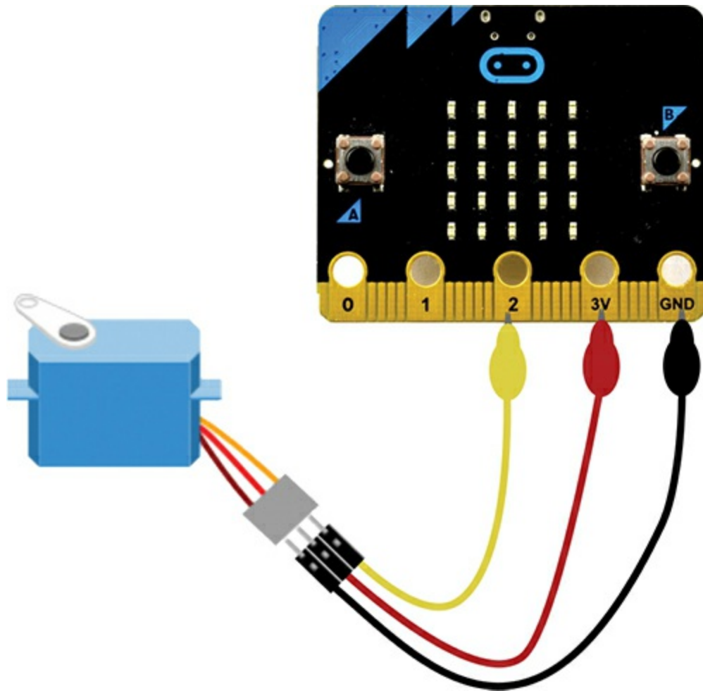
Figure 6-2: A servomotor connected to a micro:bit
