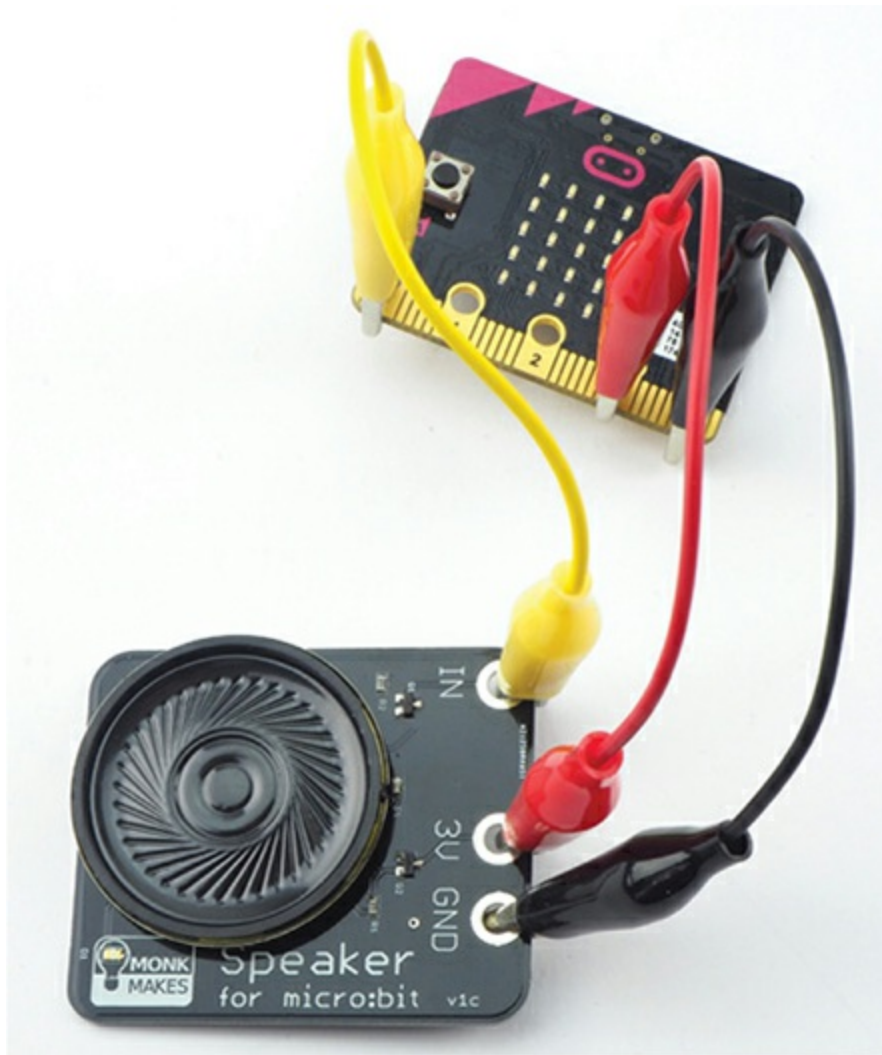
Figure 2-4: The Monk Makes Speaker for micro:bit
