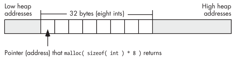
Figure 11-1: Memory allocation via malloc( sizeof( int ) * 8 )
