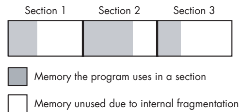
Figure 5-11: Internal fragmentation
