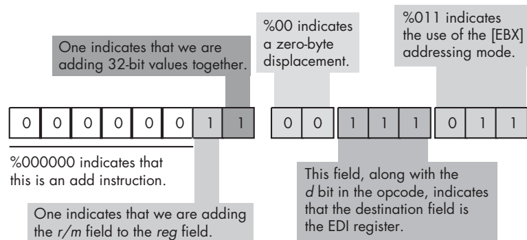
Figure 10-20: Encoding the add( disp, edx ); instruction
