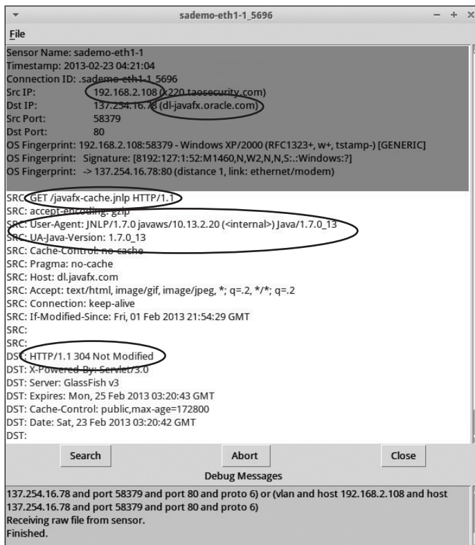
Figure 8-9: Sguil transcript
