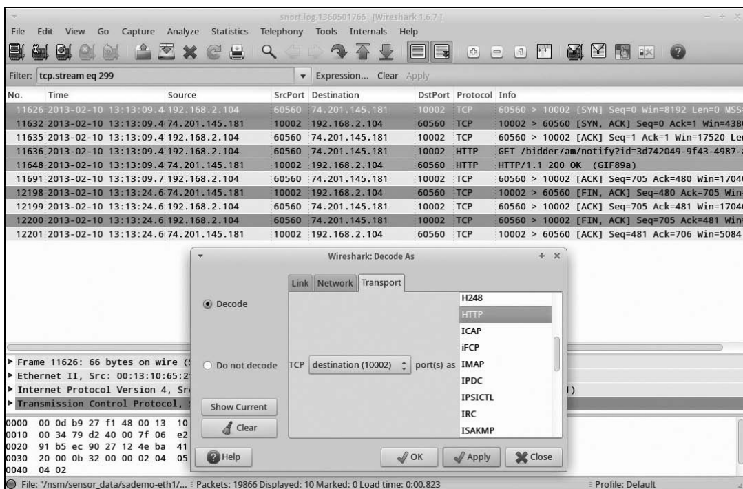
Figure 7-11: Wireshark decodes port 10002 TCP as HTTP.
