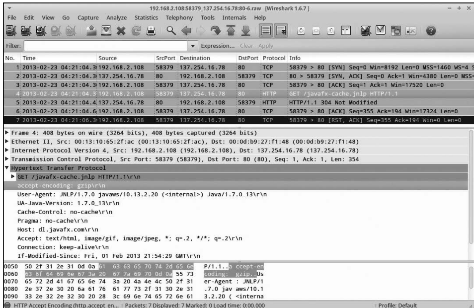
Figure 8-10: Pivoting to Wireshark from Sguil alert data
