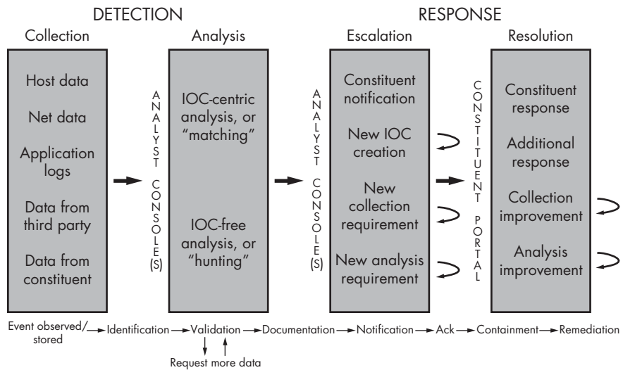
Figure 9-2: NSM process
