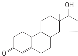
TESTOSTERONE
