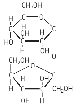
SUCROSE
