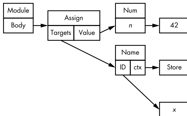
Figure 9-1: The AST of the assign command in Python
