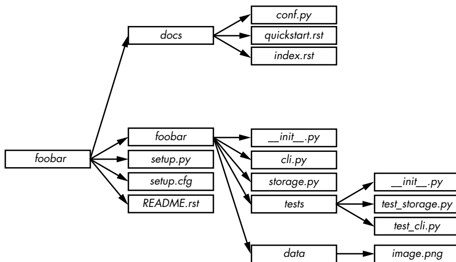
Figure 1-2: Standard package directory
