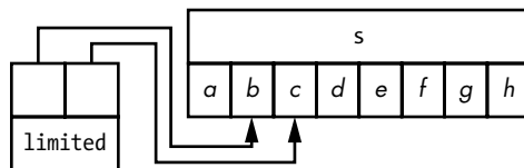
Figure 10-2: Using slice on memoryview objects
