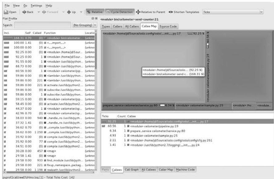
Figure 10-1: Example of KCachegrind output
