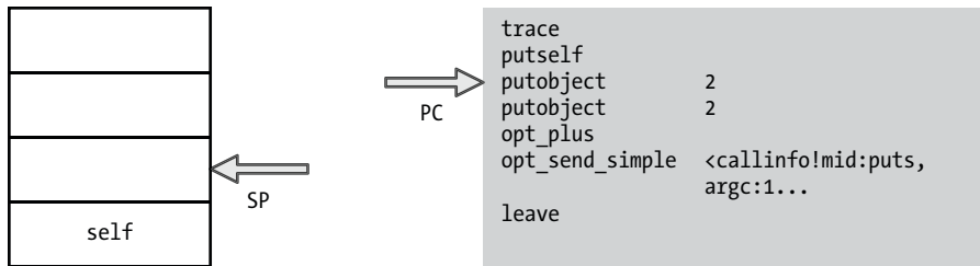
Figure 3-5: putself pushes the top self value onto the stack.
