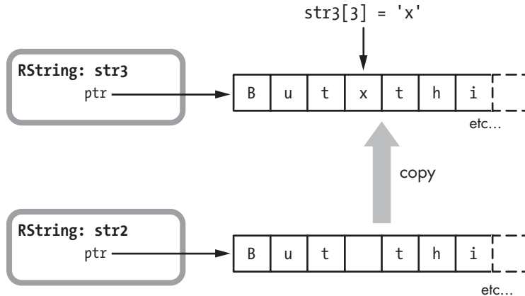
Figure 10-18: Ruby copies the string into a new buffer for str3 before writing to it.
