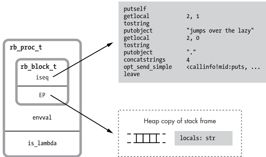
Figure 8-21: Ruby procs are closures; they contain pointers to a function and a referencing environment.
