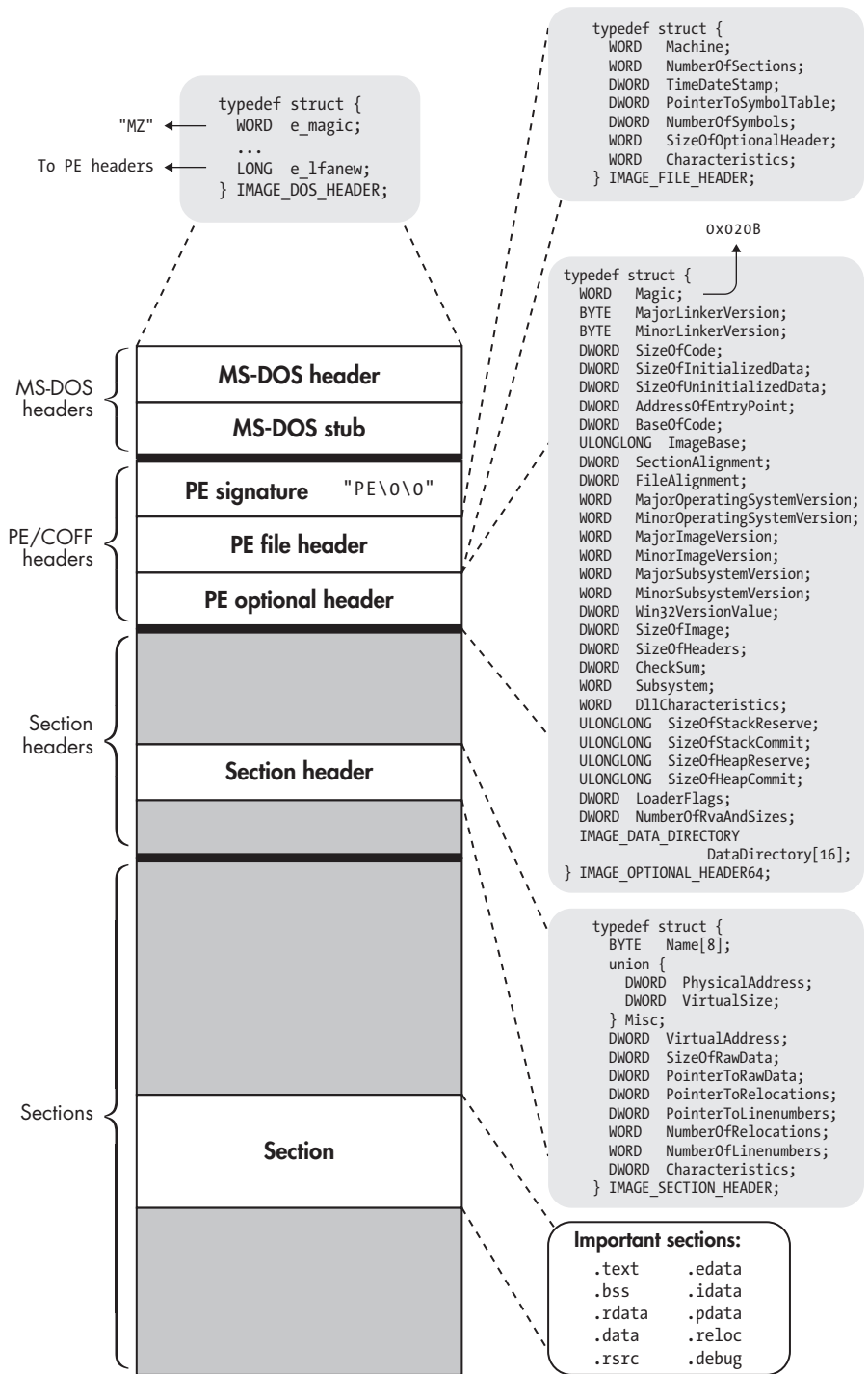
Figure 3-1: A PE32+ binary at a glance
