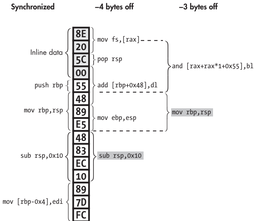
Figure 6-2: Disassembly desynchronization due to inline data interpreted as code. The instruction where the disassembler resynchronizes is shaded gray.
