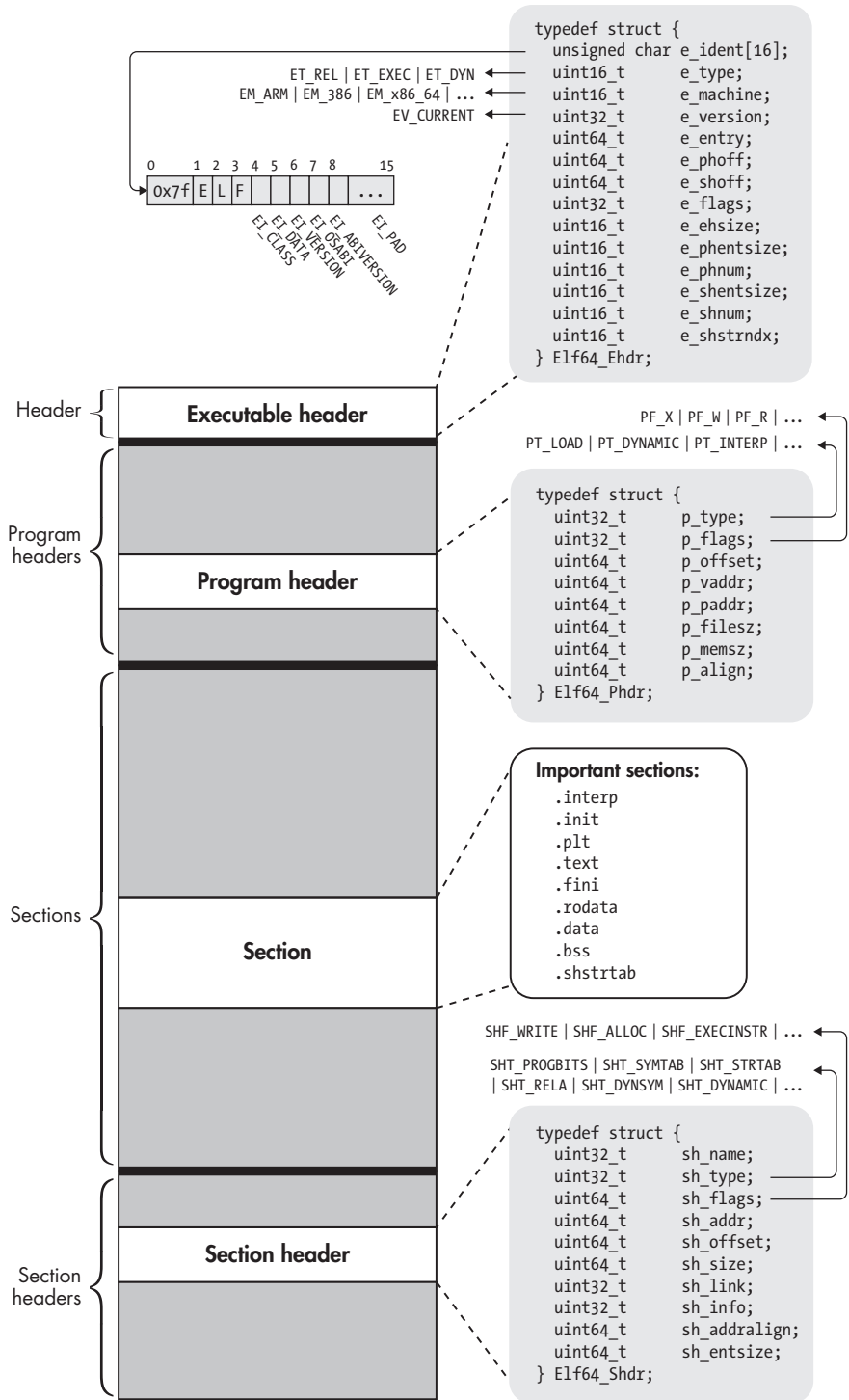
Figure 2-1: A 64-bit ELF binary at a glance
