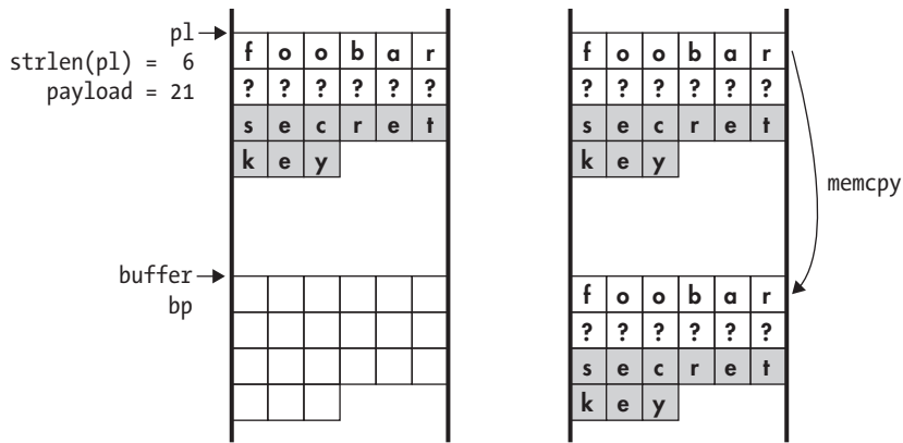
(a) A received Heartbeat request is stored in memory, next to some random data and a (tainted) secret key.
