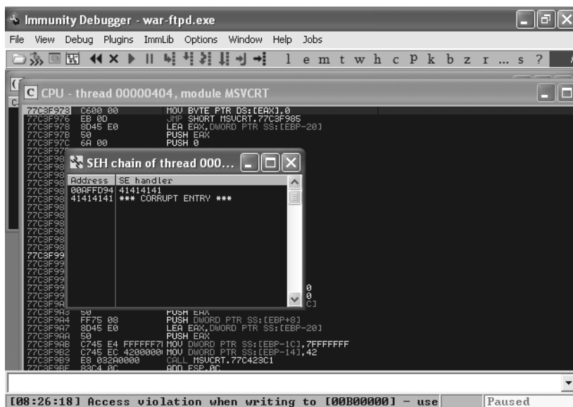
Figure 18-4: SEH overwritten
