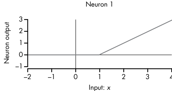
Figure 10-5: Visualization of neuron 1 as a function. The x-axis represents the neuron's single input value, and the y-axis represents the neuron's output.
