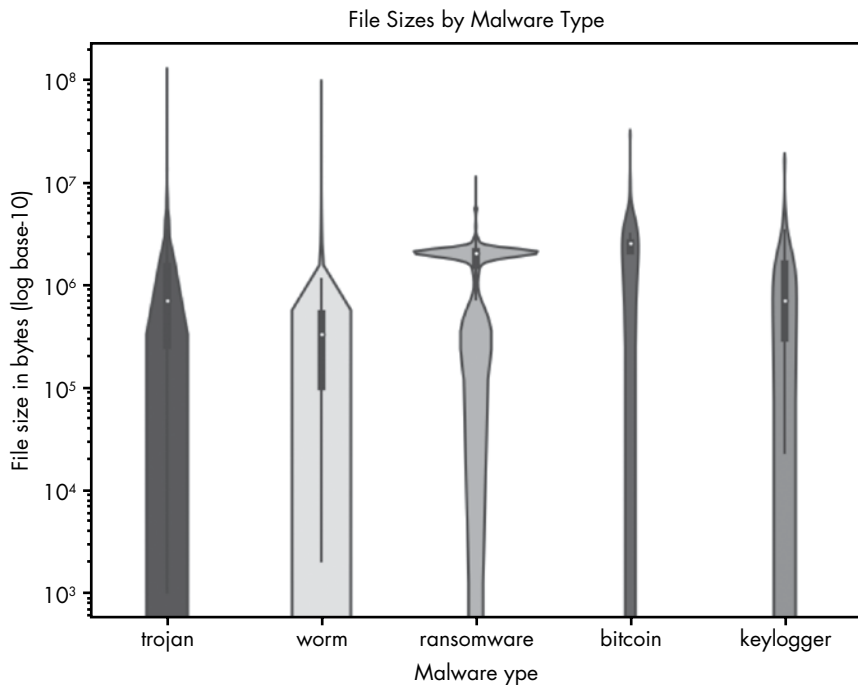
Figure 9-9: Visualization of file sizes by malware type
