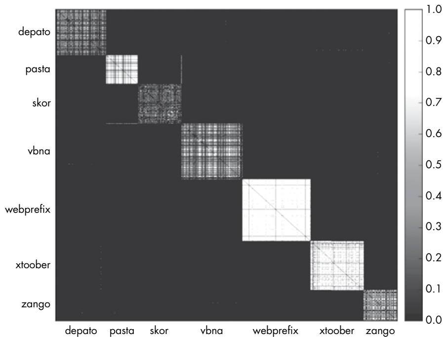
Figure 5-9: The similarity matrix generated using Import Address Table features
