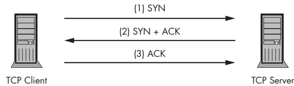
Figure 3-4: TCP three-way handshake
