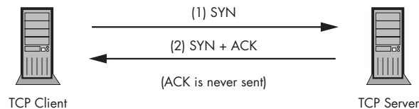
Figure 3-5: TCP half-open scan
