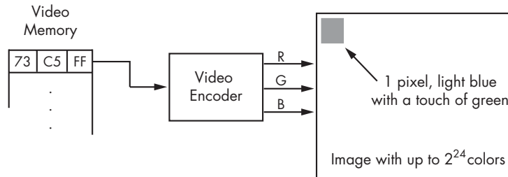
Figure 11-5: Truecolor graphics
