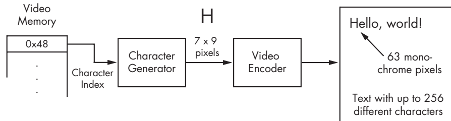
Figure 11-2: Character graphics
