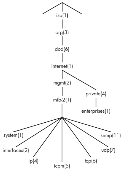
Figure 13-1: MIB-2
