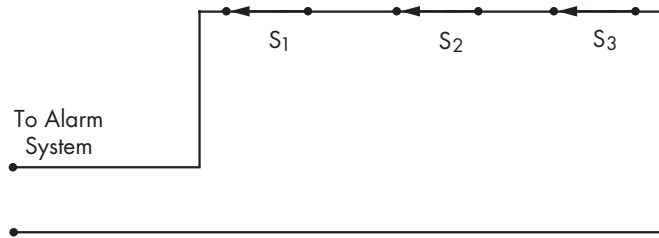
Figure 5-3: How to cascade normally closed sensors
