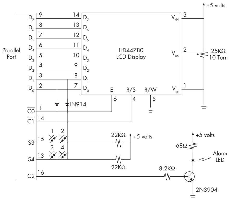
Figure 10-7: Schematic of the Laddie front panel
