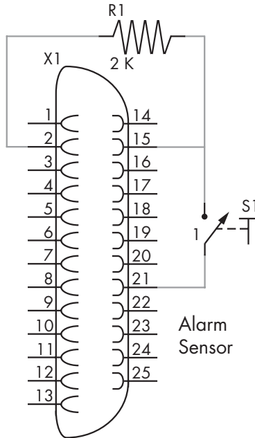
Figure 5-6: A normally open alarm sensor from Laddie
