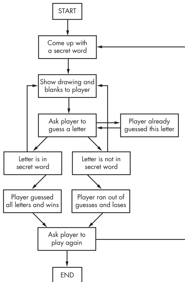
Figure 7-1: The complete flowchart for the Hangman game
