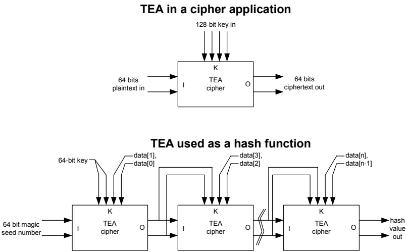
Figure 7-1: Tea cipher usage scenarios.
