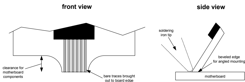
Figure 8-3: Shaping of the HyperTransport tap board edge.
