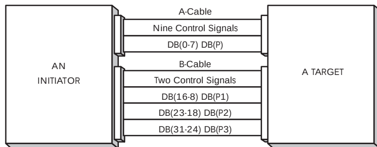
Figure 7.6: The A- and B-Cables
