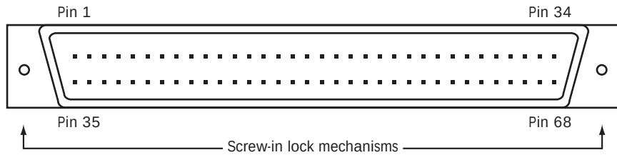
Figure A.13: Shielded High-Density Sub-D Connector, Male (Cable)
