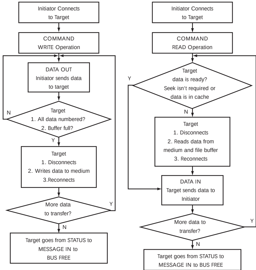
Figure 7.14: How Disconnection and Reconnection Increase I/Os
