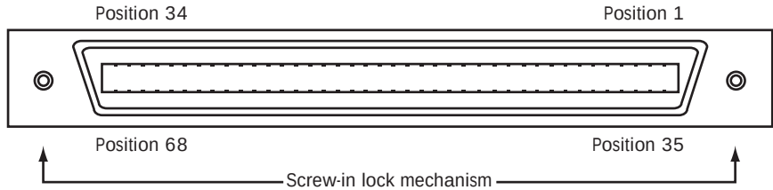
Figure A.16: VHDCI Connector, Female (Device)
