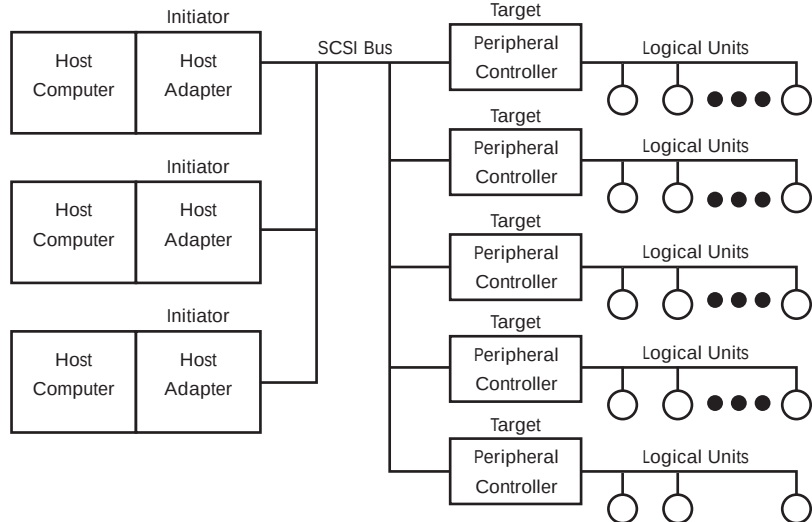
Multiple Initiators and Multiple Targets
