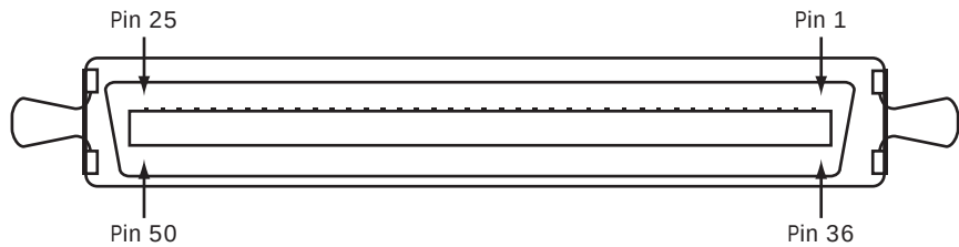
Figure A.10: Centronics-Style Low-Density Connector, Female (Device)
