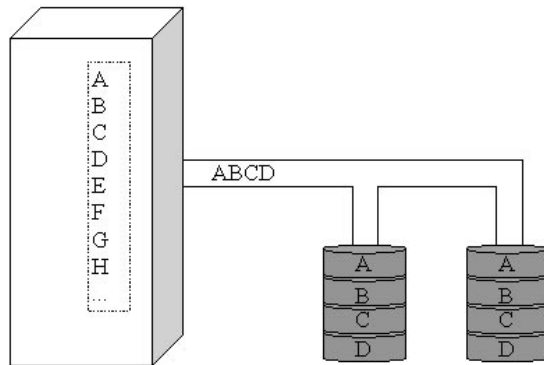
Figure 10.2: RAID 1 — Mirroring
