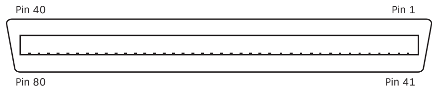
Figure A.8: SCA-2 Connector, Male (Device)
