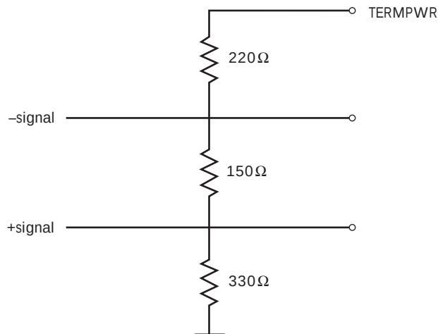
Figure A.35: Passive Termination, High Voltage Differential
