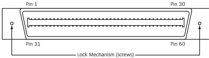
Figure A.19: IBM 60-Pin High-Density Centronics Connector, Male (Cable)
