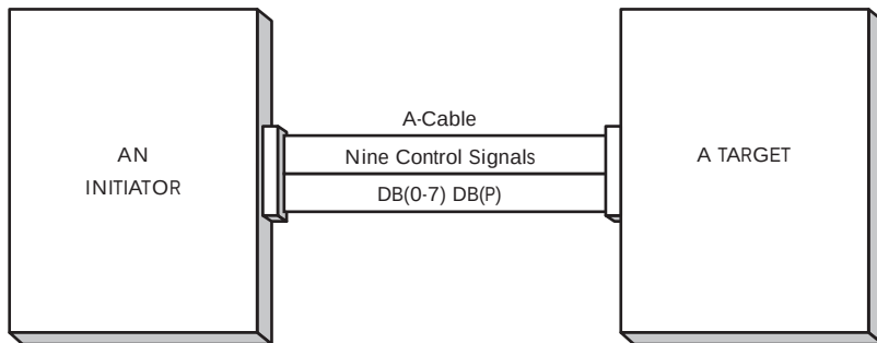
Figure 7.5: The A-Cable
