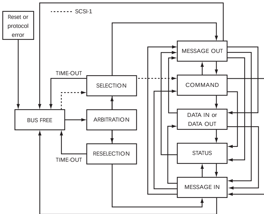
Figure 7.12: Phase Sequence Diagram
