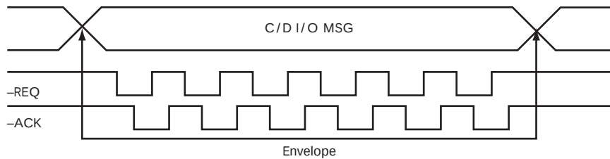
Figure 7.16: Enveloping the REQ/ACK Handshakes Until the End of the Handshake
