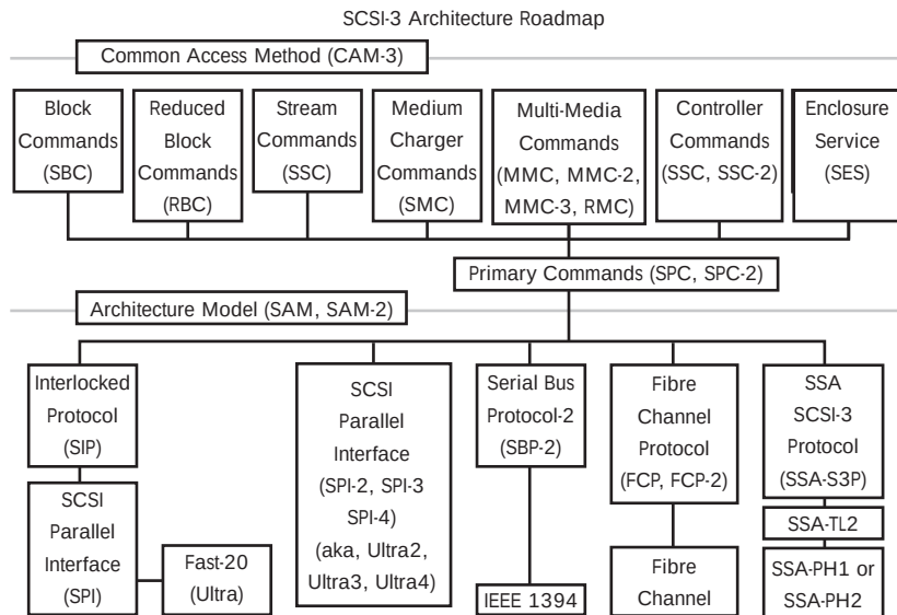
Figure 2.1: SCSI-3 Organization Chart
