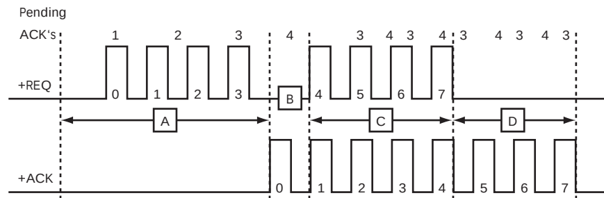
Figure 7.18: Synchronous Offset Timing Diagram
