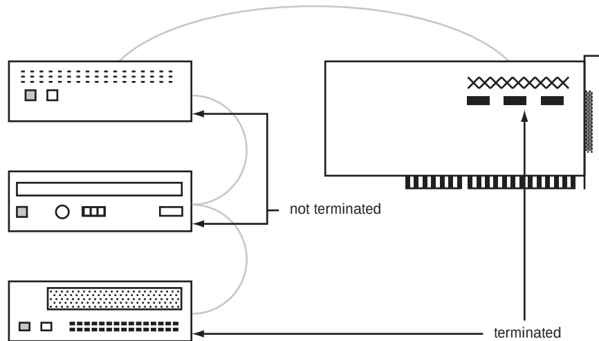
Figure A.31: Termination, Internal Devices Only
