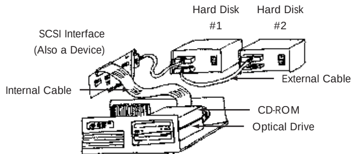
Figure 5.8: Example of a Daisy-Chained SCSI System
