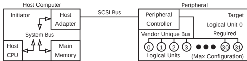
Single Initiator and Multiple Targets
