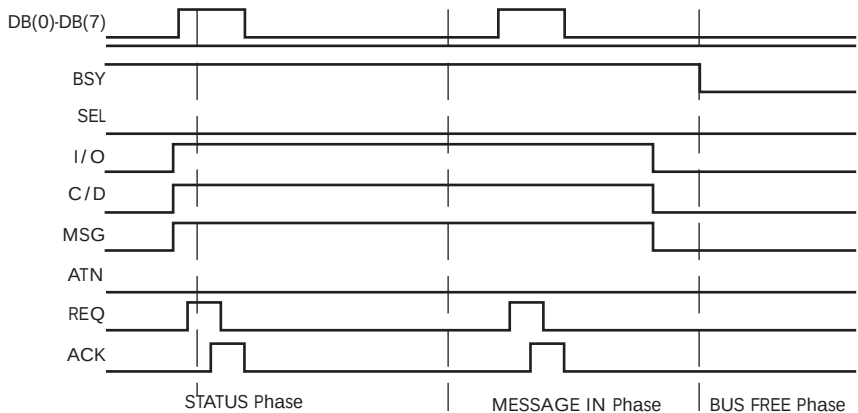
Figure A.30: MESSAGE IN Phase and BUS FREE Phase
