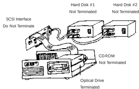
Figure 5.12: A Correctly Terminated SCSI Bus with the Host in the Middle
