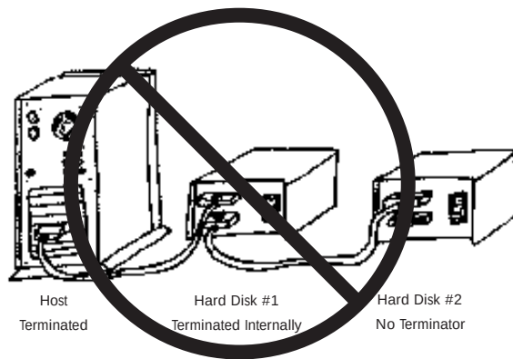
Figure 5.10: SCSI Bus Terminated in the Middle
