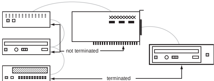
Figure A.33: Termination, Internal and External Devices
