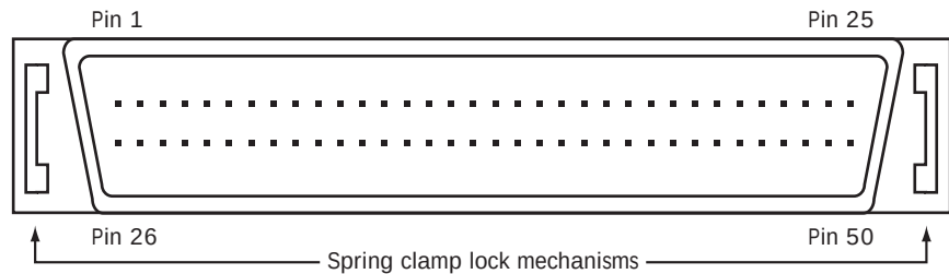
Figure A.11: Shielded High-Density Sub-D Connector, Male (Cable)
