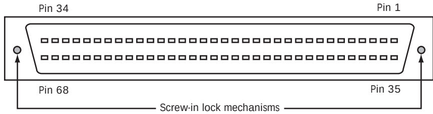
Figure A.14: Shielded High-Density Sub-D Connector, Female (Device)
