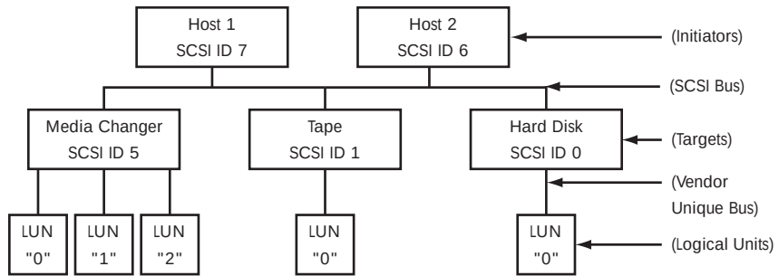
Figure 7.13: How SCSI IDs Are Used to Form a Nexus
