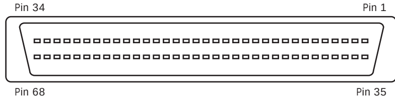
Figure A.6: SCSI-2 Wide High-Density Connector, Female (Device)
