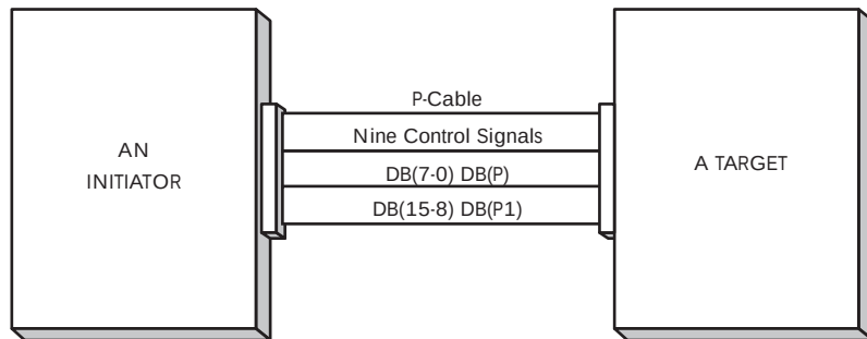
Figure 7.7: The P-Cable
