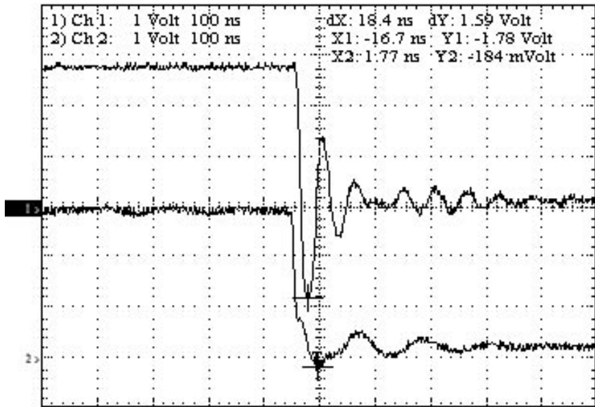
Figure 6.1: Oscilloscope View of a Signal
