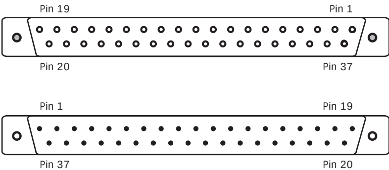
Figure A.23: Novell/Procomp 37-Pin D-Sub Connector
