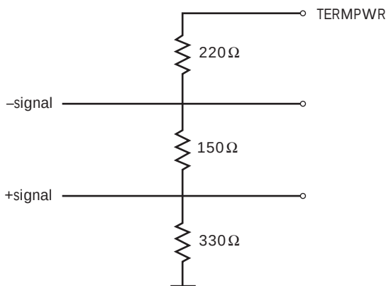
Figure 3.3: Schematic of Differential (HVD) Terminator
