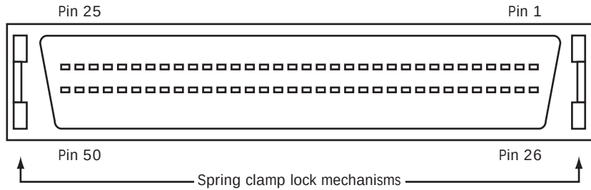
Figure A.12: Shielded High-Density Sub-D Connector, Female (Device)
