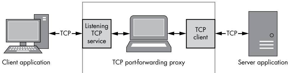
Figure 2-8: Overview of a TCP port-forwarding proxy
