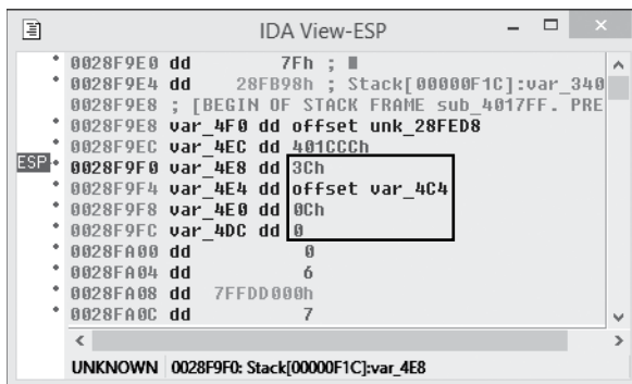
Figure 6-15: The debugger ESP window
