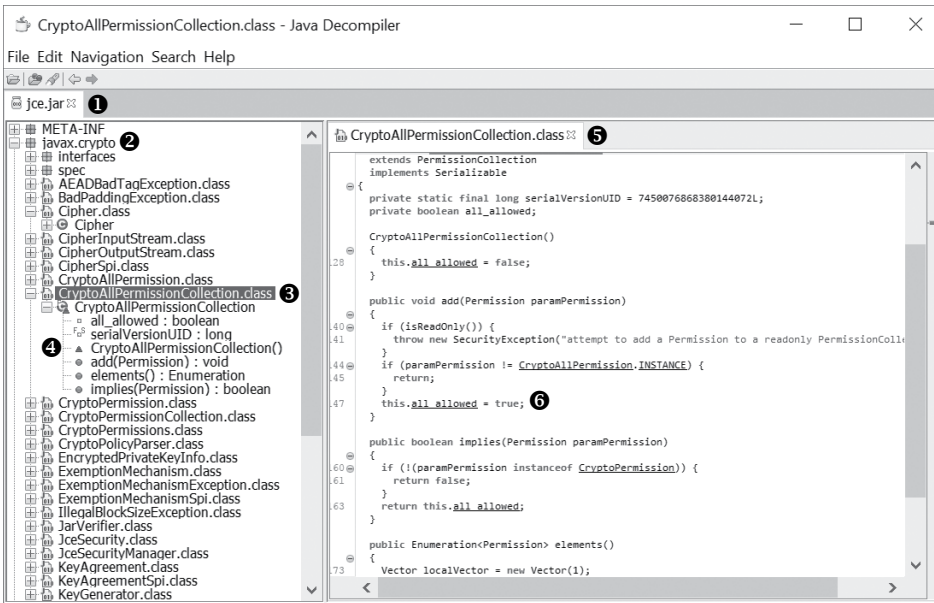
Figure 6-22: JD-GUI with an open JAR File
