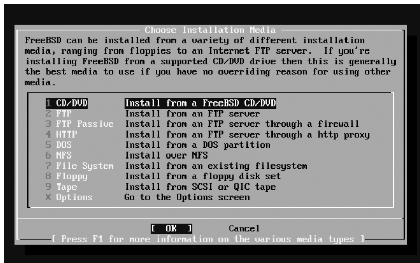
Figure 2-8: Installation media choices
