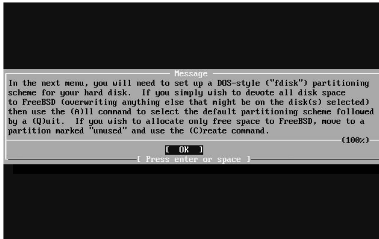
Figure 2-2: The fdisk instructions
