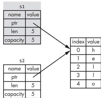
Figure 4-4: Representation in memory after s1 has been invalidated
