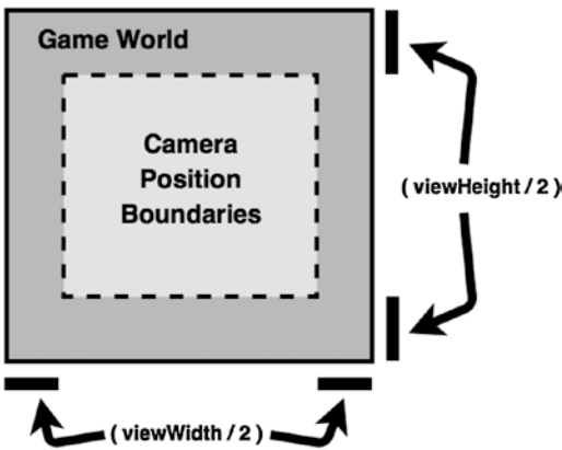
Figure 3-13. Boundaries for the camera to keep the viewing area within the game world
