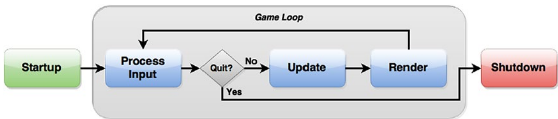
Figure 2-2. The stages of a game program
