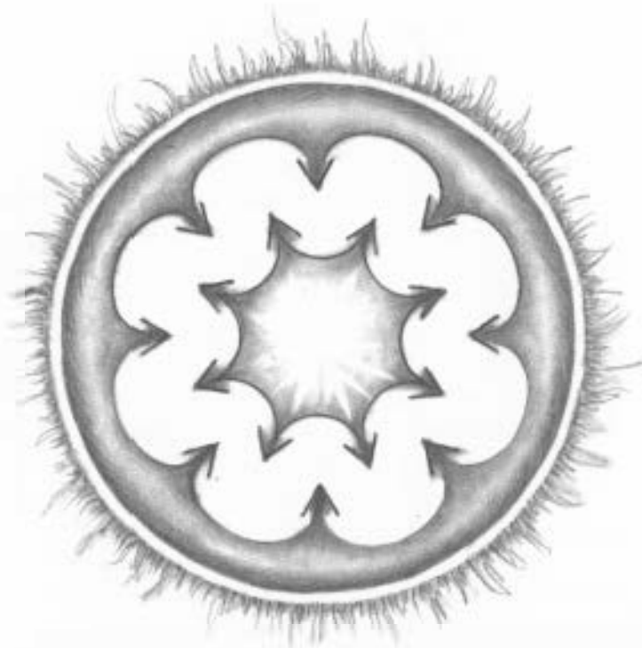
Pressure from inside the Sun balances the pull of gravity
