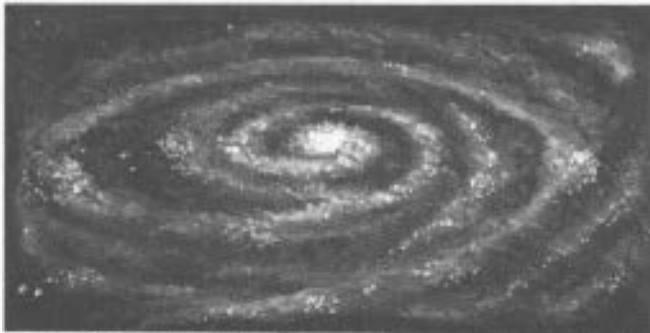
gradually coalesces
