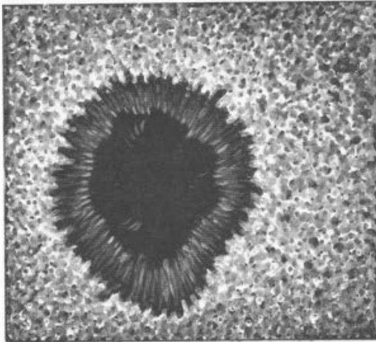
Sunspot
