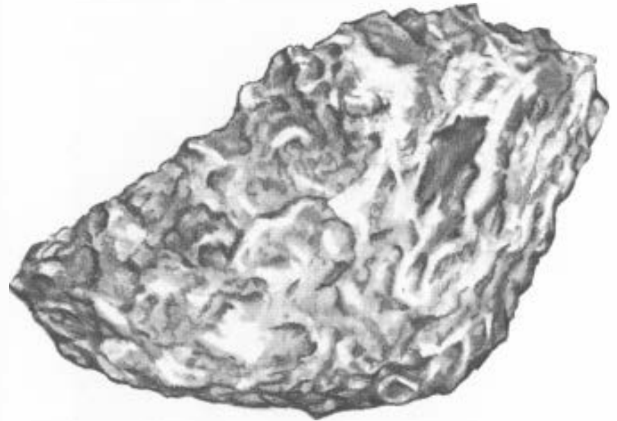
A meteorite
