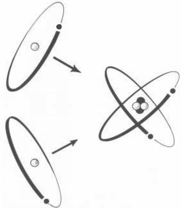
Solar fusion: two hydrogen atoms combine to form helium atom
