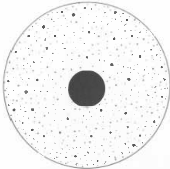
Rutherford's view of an atom
