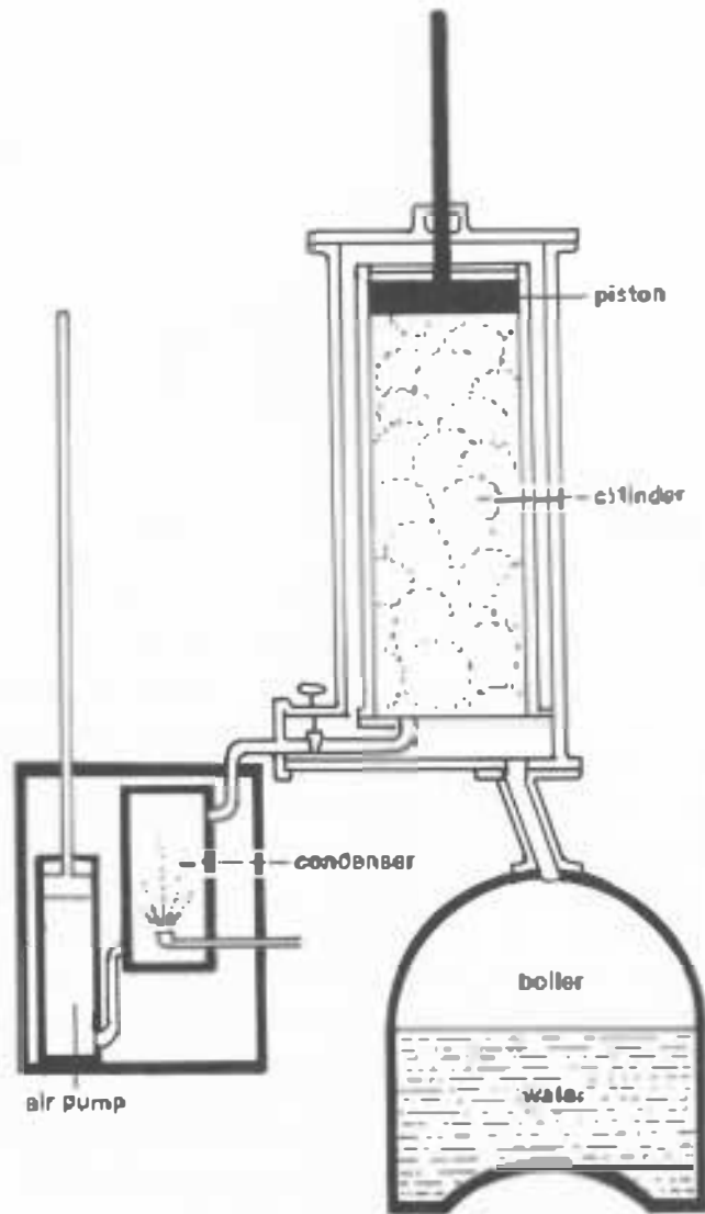
Watt's steam engine
