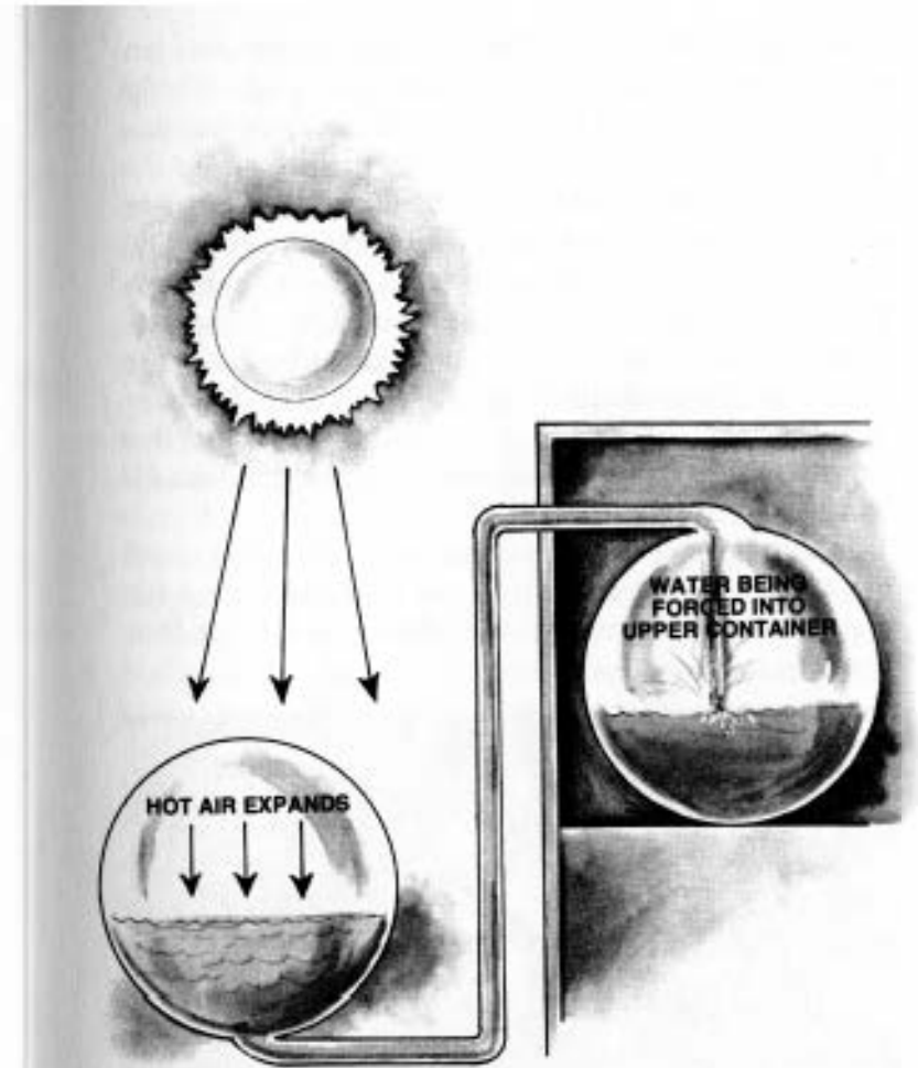
HERO'S DEVICE
