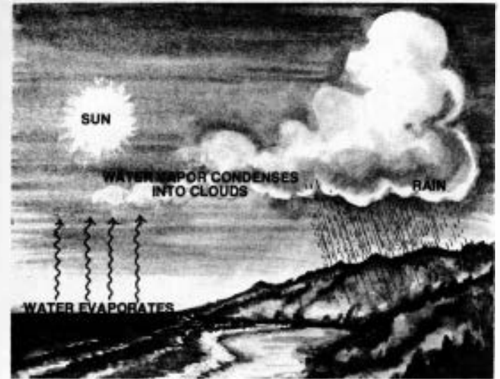
WATER CYCLE
