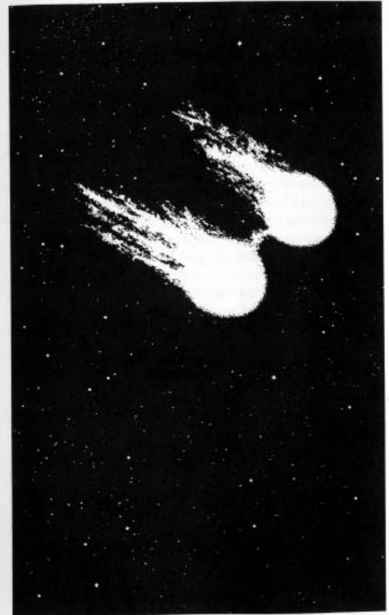
Biela's comet
