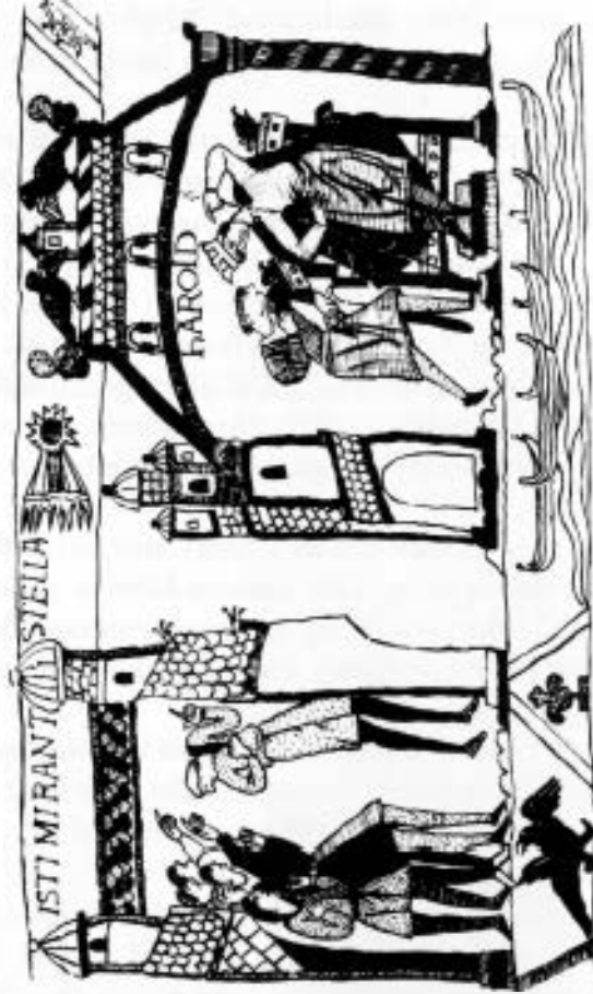
Halley's comet of 1066 AD as illustrated on the Bayeux Tapestry
